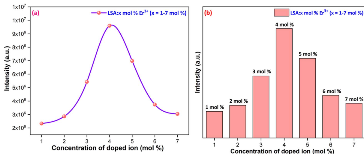
Fig. 11 Concentration quenching profiles of the considered nanophosphors.
