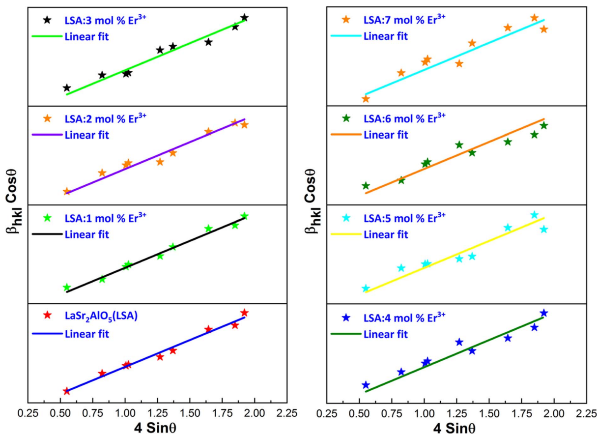
Fig. 3 W–H plot for the host and different doped \text{La}_{1-x}\text{Sr}_x\text{AlO}_5:\text{xEr}^{3+} ( x = 1-7 mol%) samples.
