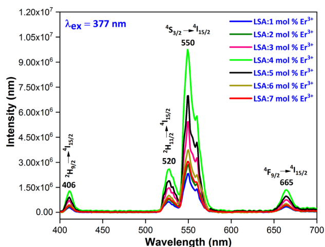
Fig. 9 Emission spectra of the \text{La}_{1-x}\text{Sr}_2\text{AlO}_5:x\text{Er}^{3+} ( x = 1-7 \text{ mol}\% \text{Er}^{3+} ) nanophosphors.
