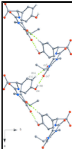
Fig. 2. The hydrogen-bonded one-dimensional helix chain of the molecule A with an R_2^2(9) ring motif viewed along the c axis. The disordered moieties and some hydrogen atoms are omitted for clarity. [Symmetry code: (i) x + 1/2, -y + 1/2, -z + 1 ].
