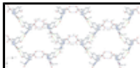
Fig. 3. The two-dimensional network of the title compound with R_2^2(8) and R_2^2(9) ring motifs viewed along the c axis. The disordered moieties and some hydrogen atoms are omitted for clarity. [Symmetry codes: (i) x + 1/2, -y + 1/2, -z + 1 ; (ii) x + 1/2, -y + 5/2, -z + 1 ].
