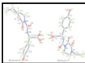
Fig. 1. A view of the title compound, showing 30% probability displacement ellipsoids. The disordered moieties (dotted lines) are shown.
