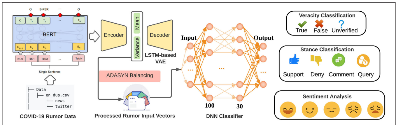
FIGURE 9 | Our rumor deep learning-based classification system. Textual sentences in our dataset are first converted to vectors using Bidirectional Encoder Representations from Transformers (BERT), and then sent through an LSTM-based Variational AutoEncoder (VAE) to extract features. After the ADASYN balancing, the processed rumor input vectors are taken by the DNN classifier as input. Three classification tasks (veracity, stance, and sentiment) are finally performed separately.
