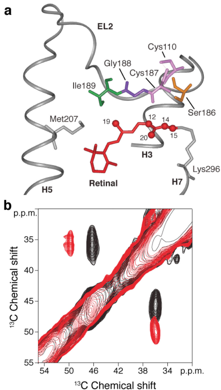
Figure 1. Structural changes involving the conserved Cys110 - Cys187 disulfide link on activation of rhodopsin. (a) View of the \beta 4 strand of EL2 from the rhodopsin crystal structure 6 highlighting the interactions of Ile189, Gly188, Cys187 and Ser186 with the polyene chain of the retinal. Cys110 on the extracellular end of H3 forms a conserved disulfide link with Cys187 in \beta 4 . (b) A region from the 2D DARR NMR spectrum of rhodopsin selectively labeled with ^{13}\text{C}\beta -cysteine. The figure highlights the crosspeak between Cys187 (46.8 ppm) and Cys110 (36.4 ppm) in rhodopsin (black). On conversion to meta II (red) there is a
