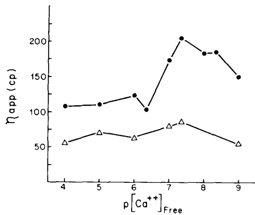
FIGURE 7 Effect of Ca^{++} on the interaction of lysosomal membrane with actin. Actin at a final concentration of 1 mg/ml was mixed with 1.5 mg/ml low-salt washed lysosomal membrane in pH 7.0 polymerization buffer at the indicated free Ca^{++} concentrations expressed as p[Ca^{++}]_{Free} . Each sample was titrated individually as described in Materials and Methods. ●, low-salt washed lysosomal membrane plus actin; \Delta , actin alone.
