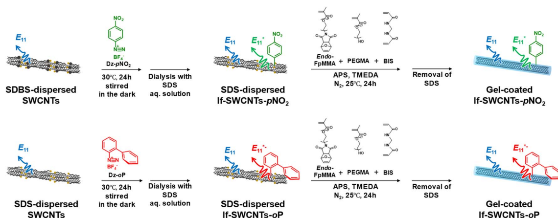
Fig. 1 Synthetic scheme of the gel-coated lf-SWCNTs- \text{pNO}_2 (upper) and gel-coated lf-SWCNTs- \text{oP} (lower).
