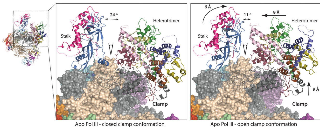
Figure 5. Conformational changes in apo Pol III
