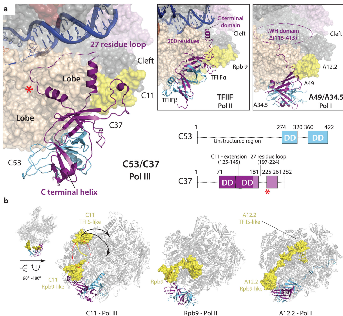
Figure 4. Architecture and Pol III-specific function of the C53/C37 heterodimer and C11 a , Model of the Pol III C53/C37 heterodimer shown in ribbon representation bound to the Pol III core (left), Pol II homologue TFIIIFα/β bound to the Pol II core (center, PDB 4v1n) and Pol I homologue A49/A34.5 bound to the Pol I core (right, PDB 4c3i). The red asterisk (left panel) marks the position of the five residues that upon deletion lead to a terminator read-through phenotype 13 . Schematic representations of C53 and C37 show the domain boundaries of the dimerization domain (DD) and additional elements. Dotted lines indicate unstructured regions. b , Conformation of subunit C11 in Pol III (left), subunit Rpb9 in Pol II (middle), and subunit A12.2 in Pol I. Subunits C11, Rpb9 and A12.2 are depicted with yellow surface rendering; C53/C37, TFIIIFα/β and A49/A34.5 are depicted in ribbon representation, all other subunits are colored in grey. Arrows indicate the potential
