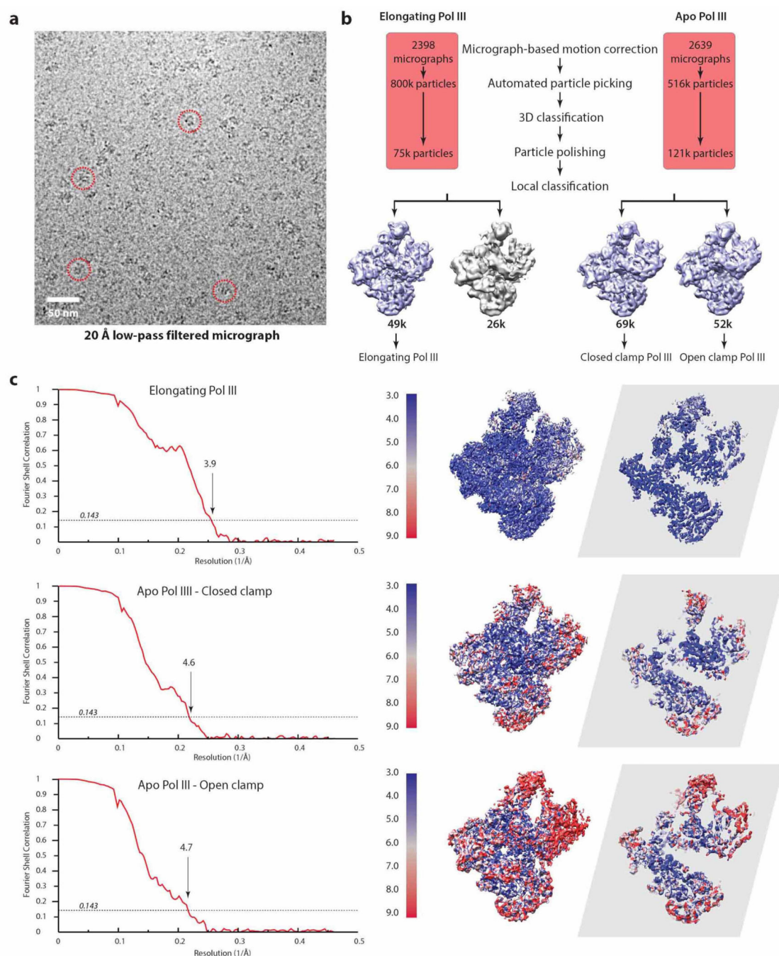
Extended Data Figure 1. Pol III processing pipeline, Fourier-shell correlation (FSC) curves and local resolution assessment
