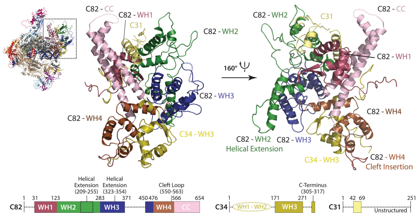
Figure 3. Architecture of the Pol III-specific heterotrimer
