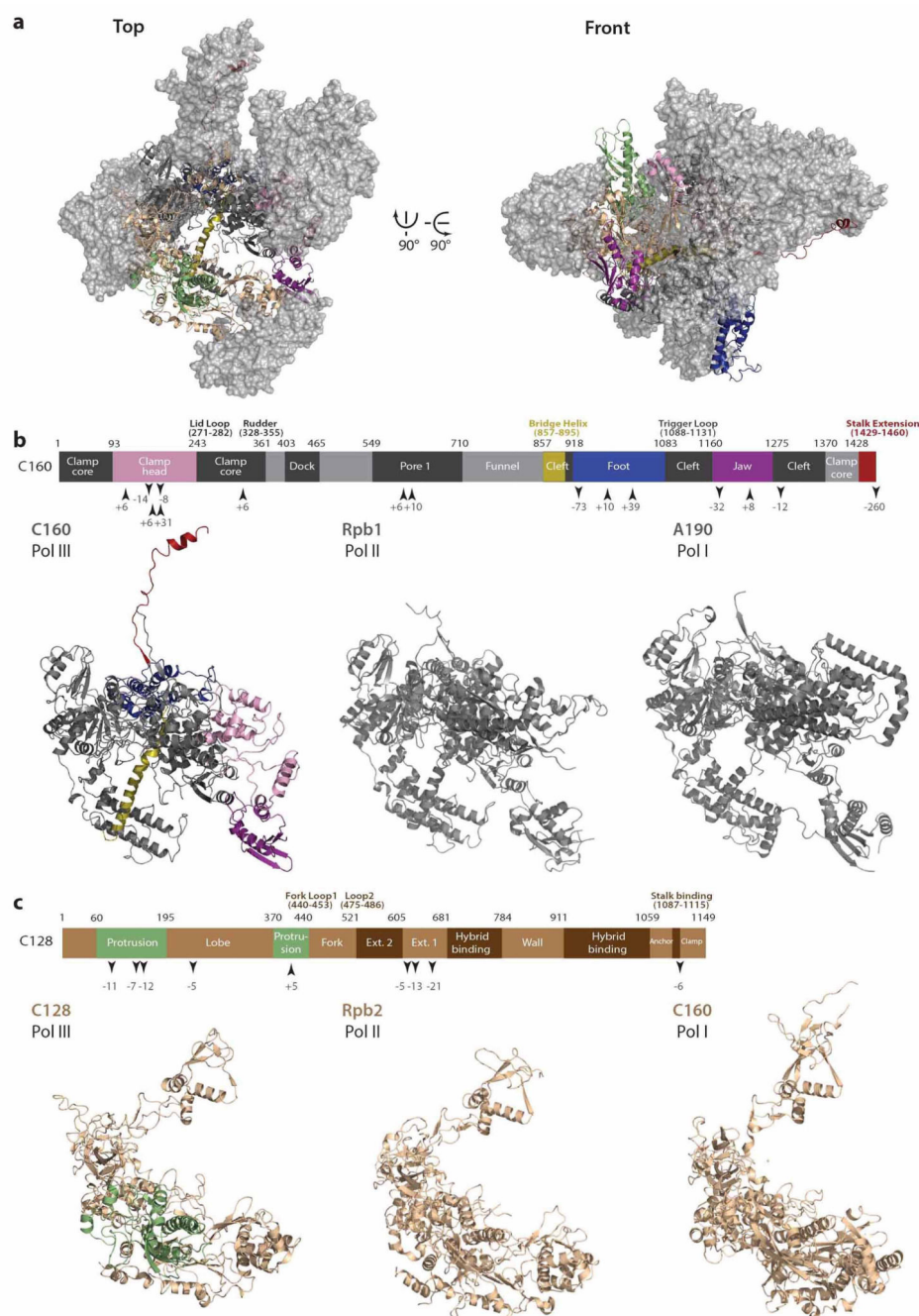
Extended Data Figure 5. Pol III-specific features of subunits C160 and C128 and comparison to the homologous Pol II and Pol I subunits
