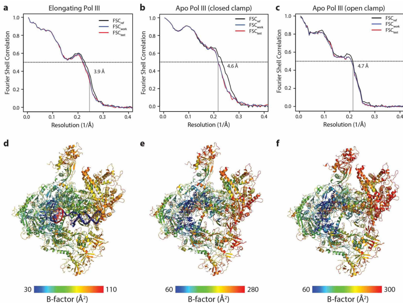
Extended Data Figure 4. Model validation and temperature factor distribution of atomic models a–c, Fourier shell correlation (FSC) curves calculated between the refined atomic model and the half map used in refinement ( FSC_{work} ) are shown in blue, those calculated between the refined atomic model and the second half map not used for refinement ( FSC_{test} ) in red. Vertical lines mark the regular FSC 0.143 cutoff and the resolution target used in refinement as shown. Close agreement between FSC_{work} and FSC_{test} and the absence of a sharp drop beyond the refinement target resolution indicate that no overfitting took place. The respective FSC between the refined atomic model and the map obtained from 3D reconstruction using the entire dataset ( FSC_{ref} ) is also shown (black). d–e, Atomic B-factor distributions mapped on ribbon representations of elongating and apo Pol III. The overall
