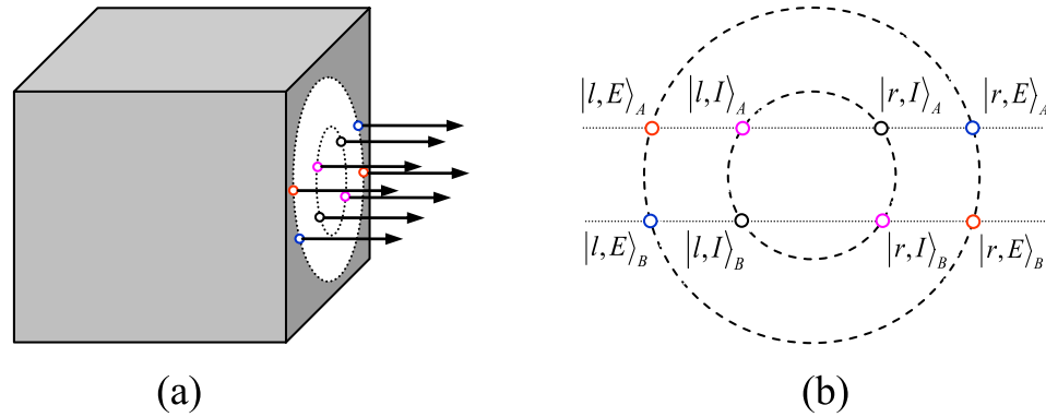
Figure 1. (a) Source for two-photon six-qubit hyperentangled Bell states. A detailed description of the source is given in the previous work 42 . (b) Modes for two-photon six-qubit hyperentangled Bell states. The upper modes correspond to Alice's photon, while the lower modes correspond to Bob's photon. l , r , I and E are the left, right, internal, and external modes for a photon, respectively.
