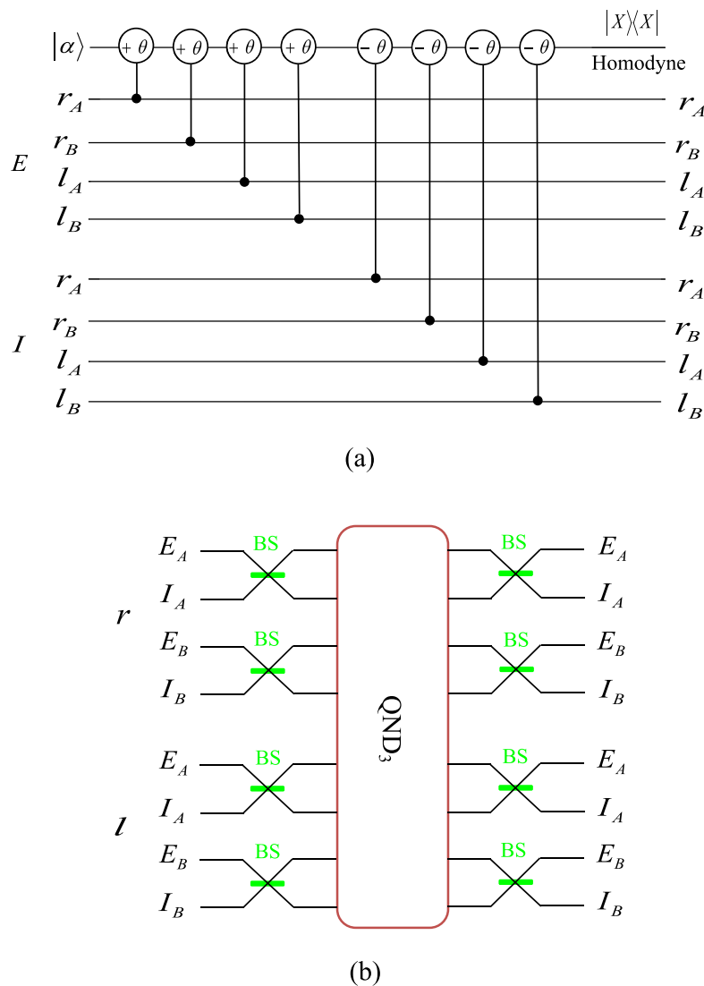
Figure 3. Schematic diagram for distinguishing the four Bell states of the two-photon six-qubit system in the second longitudinal momentum DOF. (a) QND 3 , (b) QND 4 , the 50:50 BS is used to perform the Hadamard operation ( |E\rangle \rightarrow \frac{1}{\sqrt{2}}(|E\rangle) + |I\rangle , |I\rangle \rightarrow \frac{1}{\sqrt{2}}(|E\rangle) - |I\rangle ) on the second longitudinal momentum DOF of photons.
