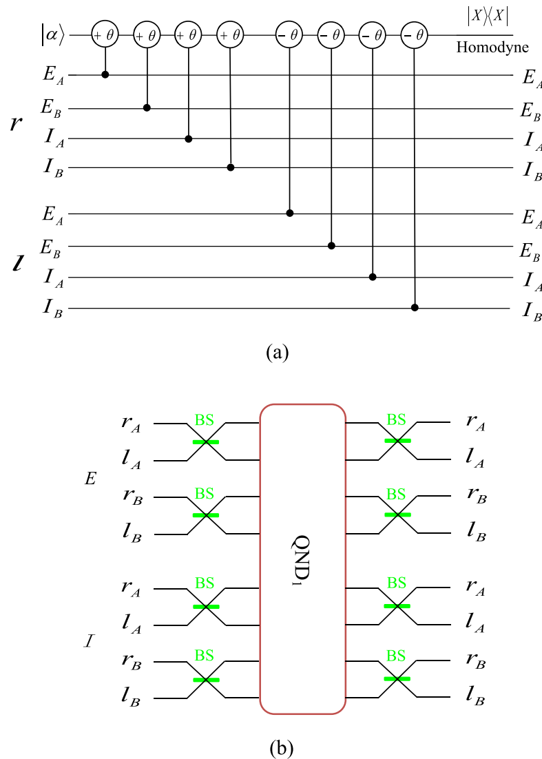
Figure 2. (a) Schematic diagram of QND 1 which is used to distinguish the even-parity states |\phi^\pm\rangle_F from the odd-parity states |\psi^\pm\rangle_F in the first longitudinal momentum DOF of the two-photon six-qubit system AB. \pm\theta denotes the cross-Kerr nonlinear media which will make the coherent probe beam |\alpha\rangle have a phase shift \pm\theta when there is a signal photon passing through it. |X\rangle\langle X| is the homodyne measurement to discriminate different phase shifts of the coherent probe beam. r and l represent the left and the right sides of each cone from where the photons emit, respectively. The internal ( I ) and the external ( E ) cones correspond to the first and the second crystal from which the photons are produced, respectively. (b) Schematic diagram of QND 2 . Each of the 50:50 BSs acts as a Hadamard operation ( |r\rangle \rightarrow \frac{1}{\sqrt{2}}(|r\rangle) + |l\rangle , |l\rangle \rightarrow \frac{1}{\sqrt{2}}(|r\rangle) - |l\rangle ) on the photon in the first longitudinal momentum DOF. After these two photons pass through the BSs, one can use mirrors to separate the paths of photons.
