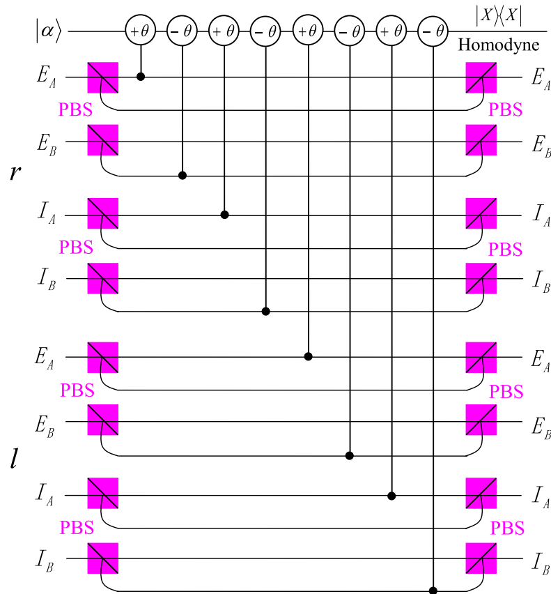
Figure 4. Schematic diagram of QND, which is used to distinguish the even-parity states |\phi^{\pm}\rangle_p from the odd-parity states |\psi^{\pm}\rangle_p in polarization DOF of the two-photon six-qubit system AB . PBS represents a polarizing beam splitter which is used to transmit the horizontal ( H ) polarization photon and reflect the vertical ( V ) polarization photon, respectively.
