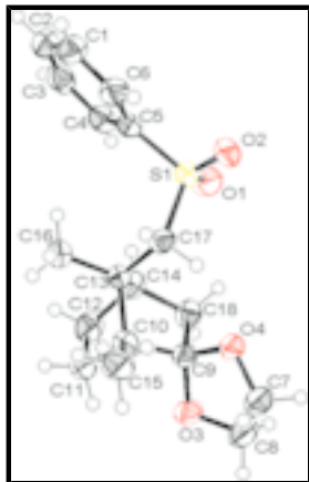
Fig. 1. The independent components of (I), showing the atom-labelling scheme. Displacement ellipsoids are drawn at the 50% probability level.
