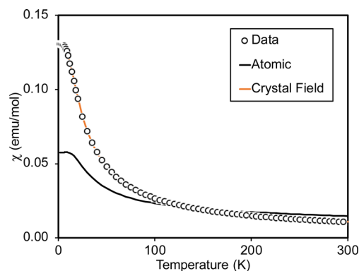
Fig. 5 Magnetic susceptibility of \text{Cp}'_3\text{Eu} (open circles). The fit using eqn (4) (free-ion model) is shown as a solid black line. The results of fitting the data using CONDON 3 (crystal field model with k = 0.7 ) is shown using an orange line.
