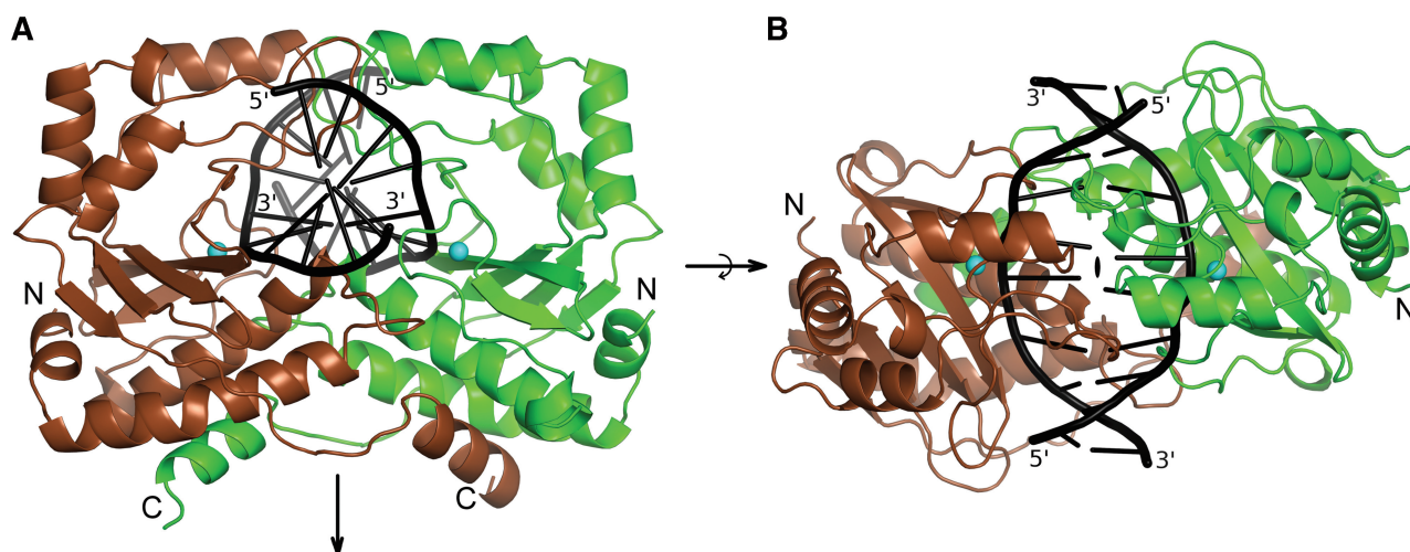
Figure 2. Overview of the ThaI –DNA complex: the two subunits of ThaI are shown in ribbon representation in green and brown color, respectively. The DNA is represented by its smoothed backbone with sticks for the bases. (A) View along the DNA. The major grooves of the central two base pairs point upwards. The 2-fold symmetry axis (arrow) of the recognition sequence and of the ThaI dimer runs vertically. In the vicinity of the central base pairs, the DNA backbone is oriented toward the viewer on the left and away from the viewer on the right side (in the 5′–3′ direction). (B) View toward the major groove of the central DNA base pairs. The two views differ by a 90° rotation about the horizontal axis.
