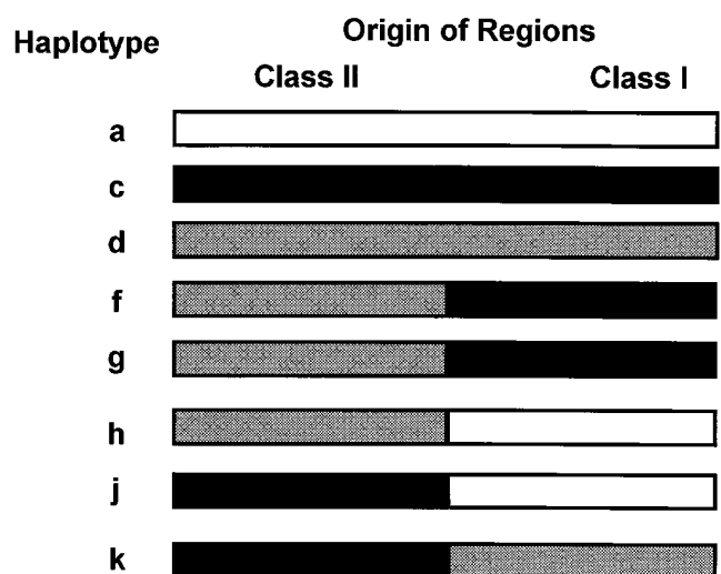
Figure 1. Schematic diagram of the origin of available homozygous porcine MHC haplotypes. Partially inbred SLA aa , SLA cc , and SLA dd haplotypes were derived from the original founder miniature swine. Recombination events between the MHC class I and class II haplotypes have been identified and maintained as homozygous, recombinant haplotypes SLA ff , SLA gg , SLA hh , SLA jj , and SLA kk .
