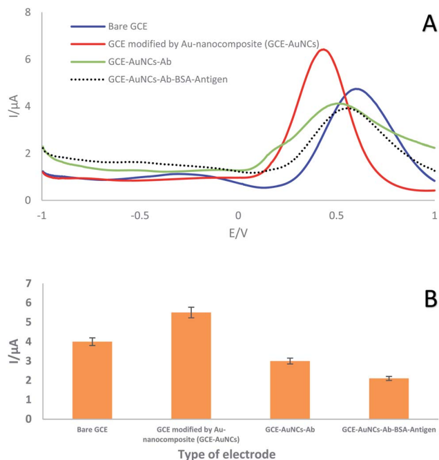
Fig. 4 (A) SWVs and (B) SWV histogram of GC electrode, GC electrode/AuNCs, GC electrode/AuNCs/Ab1 and GC electrode/AuNCs/Ab1/antigen in a solution containing 0.1 M KCl with 0.01 mol L -1 [Fe(CN) 6 ] 3-/4- as a redox probe in the potential range of -1 to +1 V ( n = 3 , S_d = 1.41 ).
