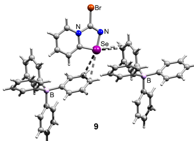
Figure 6. Ball-and-stick representation of the crystal structure of 9 , demonstrating attractive Se⋯π interactions between the selenadiazole cation and two neighboring BPh 4 anions. Grey and light-grey spheres represent carbon and hydrogen, respectively.
