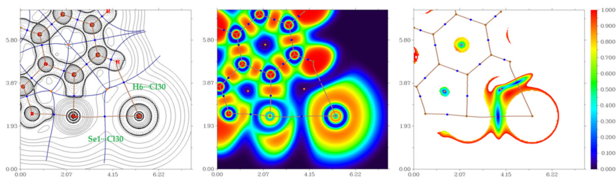
Figure 9. Contour line diagram of the Laplacian of electron density distribution \nabla^2\rho(r) , bond paths, and selected zero-flux surfaces (left panel), and visualization of electron localization function (ELF, center panel) and reduced density gradient (RDG, right panel) analyses for non-covalent interactions H6...Cl30 and Se1...Cl30 in the model supramolecular associate 4 . Bond critical points (3, −1) are shown in blue, nuclear critical points (3, −3) in pale brown, ring critical points in orange. Bond paths are shown as pale brown lines, length units are in Å, and the color scale for the ELF and RDG maps is presented in a.u. The numeration of atoms corresponds to their ordering in the attached xyz-files for model supramolecular associates (Supplementary Materials).
