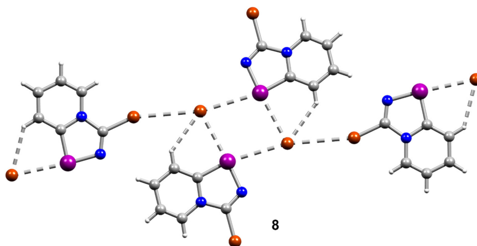
Figure 5. Ball-and-stick representation of the crystal structure of 8 , demonstrating its self-assembly into 1-D supramolecular polymer via Se⋯Br and Br⋯Br interactions. Brown, purple, blue, grey, and light-grey spheres represent bromine, selenium, nitrogen, carbon, and hydrogen, respectively.
