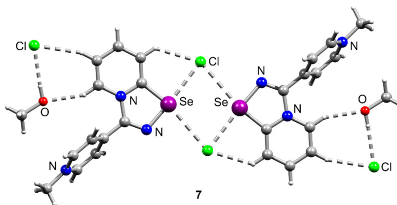
Figure 7. Ball-and-stick representation of the crystal structure of 7 , demonstrating attractive Se···Cl, H···Cl, and H···O interactions. Grey and light-grey spheres represent carbon and hydrogen, respectively.
