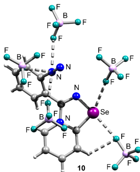
Figure 8. Ball-and-stick representation of the crystal structure of 10 , demonstrating attractive Se···F, H···F, and N···F interactions. Grey and light-grey spheres represent carbon and hydrogen, respectively.
