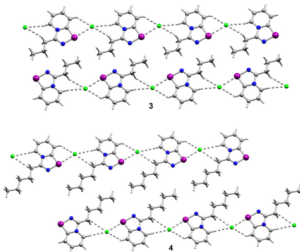
Figure 2. Ball-and-stick representations of the crystal structures of 3 and 4, demonstrating their self-assembly into 1-D supramolecular polymers via Se...Cl and H...Cl interactions. Green, purple, blue, grey, and light-grey spheres represent chlorine, selenium, nitrogen, carbon, and hydrogen, respectively.
