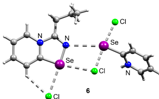
Figure 3. Ball-and-stick representation of the crystal structure of 6 , demonstrating attractive Se...N, Se...Cl, and H...Cl interactions. Grey and light-grey spheres represent carbon and hydrogen, respectively.
