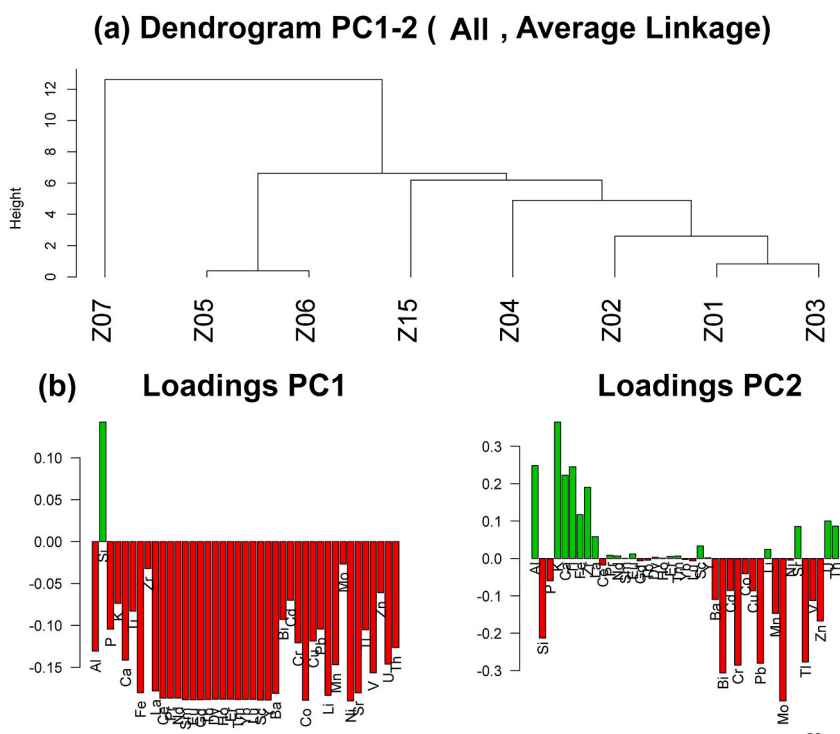
Fig. 4. CA(a) and variables/loadings plots (b) for Z01-Z07 samples employing all elements. PC1 (67.2 %) and PC2 (14.7%) explain the 81.9% of the total variance.
