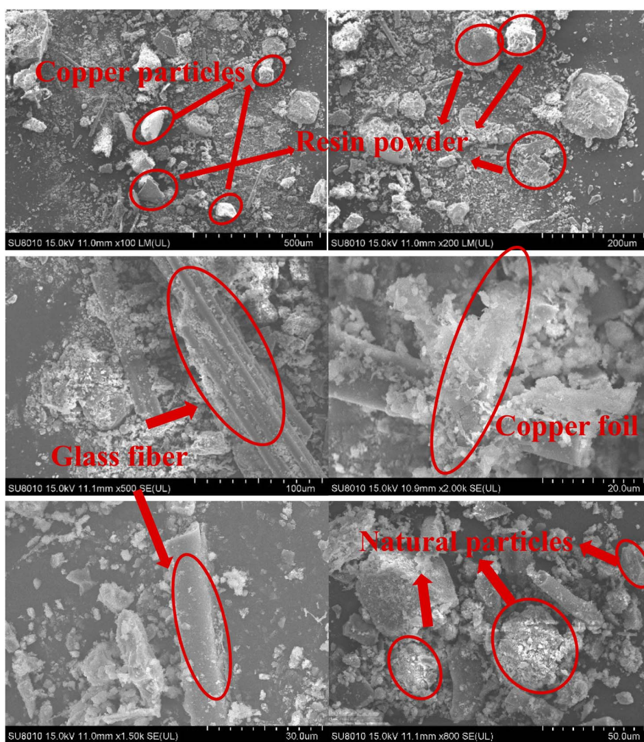
Fig. 2 SEM image of dust in the workshop.
