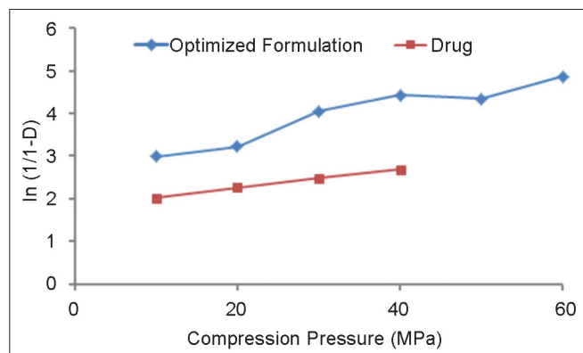
Figure 8: Heckel plots of drug and optimized agglomerates
