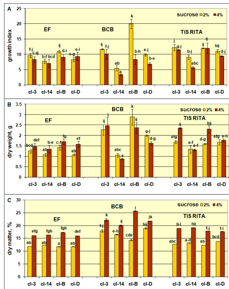
Figure 2. Growth index (A), dry weight (B), and percentage of dry matter (C) of Gentiana dinarica hairy root clones cl-3, cl-14, cl-B, and cl-D, after 7 weeks of cultivation in Erlenmeyer flasks (EF), bubble column bioreactor (BCB), and temporary immersion systems (TIS) RITA ® . Presented values are mean \pm SE of 3–6 replicates. Within each parameter, values with the same letter are not significantly different at the p \leq 0.05 level according to Fisher's least significant difference (LSD) test.
