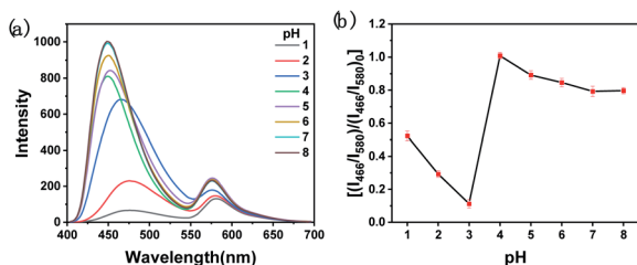
Fig. 3 (a) Fluorescence spectra of the ratiometric fluorescent probes at pH from 1 to 8. (b) Effect of pH on the detection of \text{NO}_2^- by the ratiometric fluorescent probe ( I_{466}/I_{580} is the fluorescence intensity ratio with 40 \mu\text{M NO}_2^- and (I_{466}/I_{580})_0 is without \text{NO}_2^- ). Concentration: \text{NO}_2^- , 40 \mu\text{M} ; PBS: 30 \text{ mM} , \text{pH} = 3 .
