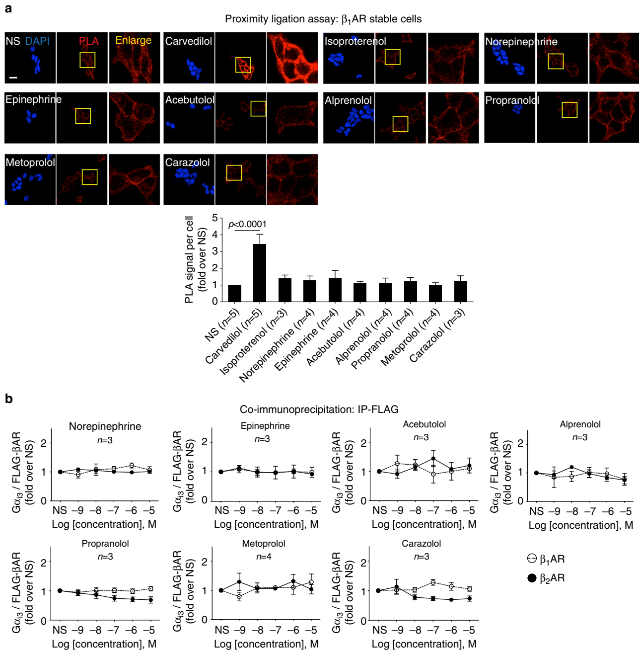
Fig. 4 A number of \beta AR agonists or antagonists tested do not have significant effect on G\alpha_i recruitment. a \beta_1 AR stable cells were stimulated with vehicle or 10 \mu\text{M} indicated ligands for 5 min. Interaction of \beta_1 AR and G\alpha_i were detected by PLA. Scale bar = 20 \mu\text{m} . b \beta_1 AR or \beta_2 AR stable cells were stimulated with ligands at indicated concentration for 5 min. G\alpha_i recruitment was detected by co-immunoprecipitation. Both assays suggested that none of the ligands tested had similar effect of carvedilol on G\alpha_i recruitment. Data represent the mean \pm SEM for n independent experiments as marked on the figure. Statistical significance vs. unstimulated cells was assessed using one-way ANOVA with Bonferroni correction
