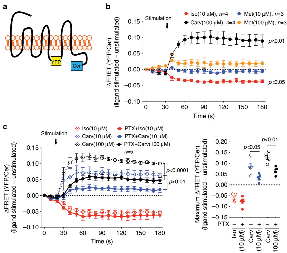
Fig. 2 G\alpha_i is required for carvedilol-induced \beta_1 AR conformation change. a In the FRET-based \beta_1 AR conformation sensor, YFP and Cerulean (Cer) are inserted in the third intracellular loop and the C-tail of \beta_1 AR respectively. b Ligand-induced changes of the FRET ratio in HEK293 cells stably expressing \beta_1 AR FRET sensor. The stable cells were stimulated with 100 \mu M carvedilol, 10 \mu M isoproterenol, 10 \mu M or 100 \mu M \beta_1 AR antagonist metoprolol, while FRET was monitored in real-time as the emission ratio of YFP to Cer. Carvedilol stimulation increased the FRET ratio, while isoproterenol decreased it, demonstrating the distinct \beta_1 AR conformations induced by these two ligands. Metoprolol had no effect on the FRET ratio. c Effect of PTX on ligand-induced FRET ratio change. Cells were pretreated with vehicle or 200 ng per ml PTX for 16 h before ligand stimulation. PTX blocked carvedilol-induced change, while having no effect on the isoproterenol response, suggesting that G\alpha_i is required to stabilize the carvedilol-induced \beta_1 AR conformation. Data represent the mean \pm SEM for n independent experiments as marked on the figure. Statistical significance vs. unstimulated cells was assessed using one-way ANOVA with Bonferroni correction ( b ); statistical significance between PTX-pretreated and non-pretreated cells was assessed using two-way ANOVA with Bonferroni correction ( c , left panel), or two-tailed paired Student's t -test ( c , right panel)
