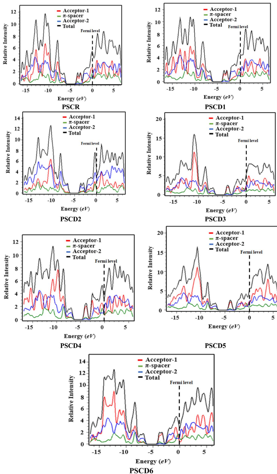
Fig. 4 DOS plots for PSCR and PSCD1–PSCD6.
