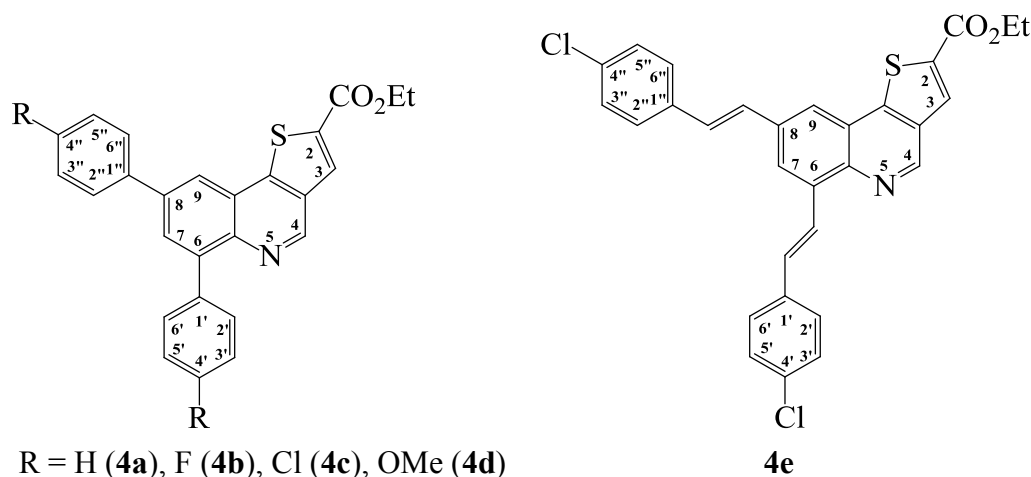
Scheme 4. Generalized structures for the ethyl thieno[3,2- c ]quinoline-2-carboxylates 4a–d and 4e .
