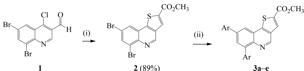
Scheme 1. Suzuki-Miyaura cross-coupling of specially prepared 2 to afford 3a–e .
