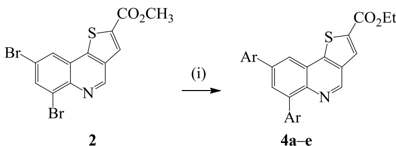
Scheme 2. One-pot Suzuki-Miyaura cross-coupling and trans-esterification of 2 to afford 4a–e .
