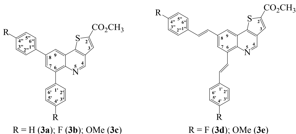
Scheme 4. Generalized structures for the ethyl thieno[3,2- c ]quinoline-2-carboxylates 4a–d and 4e .
