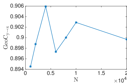
(b) (x, y) \sim U([-1.5, 1.5]^2)
