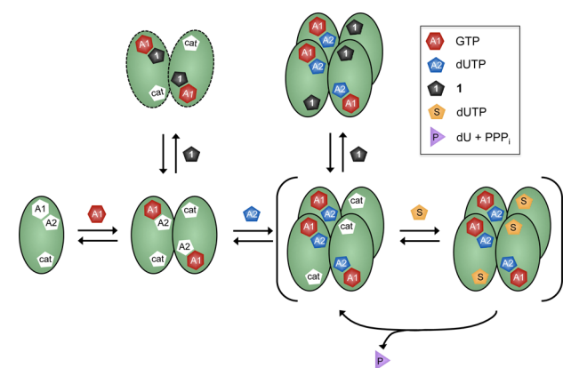
Figure 2. Double hit inhibition mechanism of 1 . Compound 1 intercepts the ordered-essential site activation mechanism of SAMHD1 by binding to the A2 activator site in a nonproductive manner that cannot lead to tetramer formation ( K_i = 50 \mu\text{M} ). In addition, 1 binds to the catalytic site and competitively inhibits substrate binding. Binding of the GTP activator to the A1 site is required to assemble dimers and to form the A2 site. The scheme also depicts the previously determined mechanistic feature where SAMHD1 turns over without release of bound activator nucleotides (brackets).
