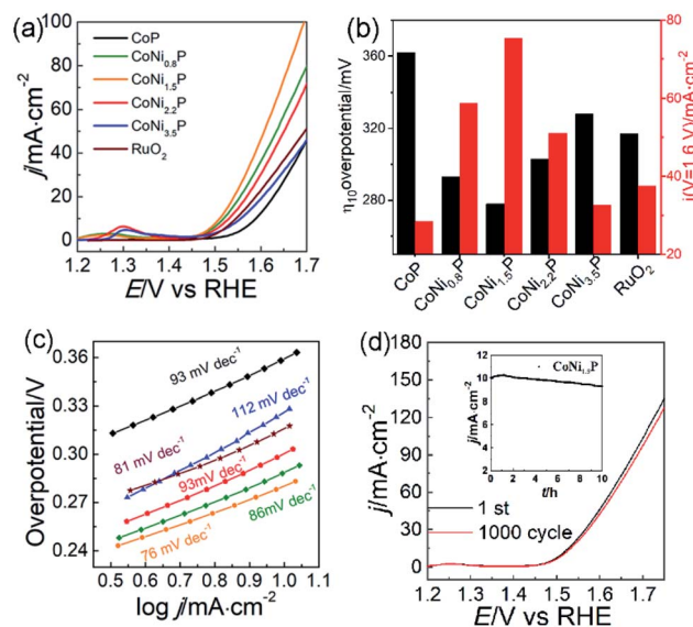
Fig. 4 (a) LSV curves, (b) summary of the overpotential at a current density of 10 \text{ mA cm}^{-2} and current density at 1.6 \text{ V} potential, (c) Tafel slopes of \text{CoP} , \text{CoNi}_{0.8}\text{P} , \text{CoNi}_{1.5}\text{P} , \text{CoNi}_{2.2}\text{P} , \text{CoNi}_{3.5}\text{P} and \text{RuO}_2 catalysts in \text{O}_2 -saturated 1.0 \text{ mol L}^{-1} KOH, (d) LSV curves of \text{CoNi}_{1.5}\text{P} before and after 1000 cycles (inset: chronoamperometry curve of \text{CoNi}_{1.5}\text{P} at an overpotential of 278 \text{ mV} over 10 \text{ h} ).
