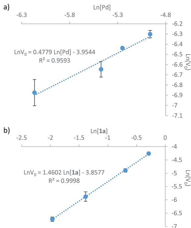
Fig. 3 Dependence of the initial rate of 5-hexynoic acid cyclization on the concentration of palladium (a) and substrate (b). The rates were averaged over three independent measurements. The error bars represent the standard deviation of the results from the three independent measurements.
