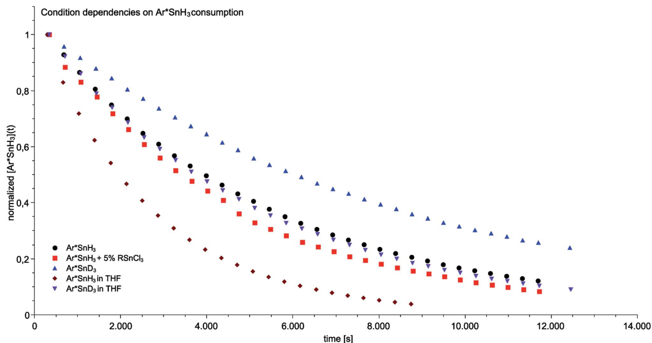
Fig. 3 Condition-dependent consumption of tin trihydride/trideuteride ( 0.046 mol L -1 ) in the course of the catalytic dehydrogenation in the presence of a six fold excess of DMAP at 40 °C determined by 1 H NMR spectroscopy.
