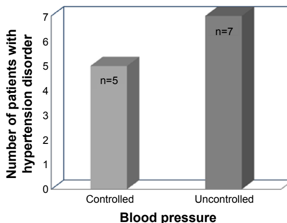
Figure 2 Cabergoline safety. Note: Total patients n=85, patients with blood pressure disorder n=12.
