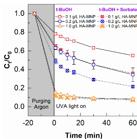
Figure 9. The removal of As(III) in the presence of \bullet\text{OH} and ^3\text{HA} - \text{MNP}^* quenchers and in the absence of molecular oxygen during photo-irradiation for 60 min. [\text{As(III)}]_0 = 200 \mu\text{g L}^{-1} , [\text{HA} - \text{MNP}] = 0.1, 0.2, and 1.0 \text{ g L}^{-1} , [t\text{-BuOH}] = 10 \text{ mM} , and [\text{sorbate}] = 10 \text{ mM} ; error bars represent the standard deviation of triplicate measurements.
