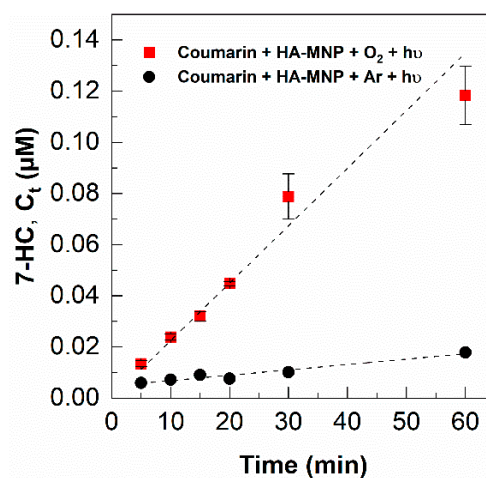
Figure 3. Formation of 7-HC in the presence of UVA and [\text{HA-MNP}] = 1.0 \text{ g L}^{-1} ; [\text{Cou}]_0 = 125 \text{ }\mu\text{M} , oxygen-saturated (■) and argon-saturated (●) environments; error bars represent the standard deviation of triplicate measurements.
