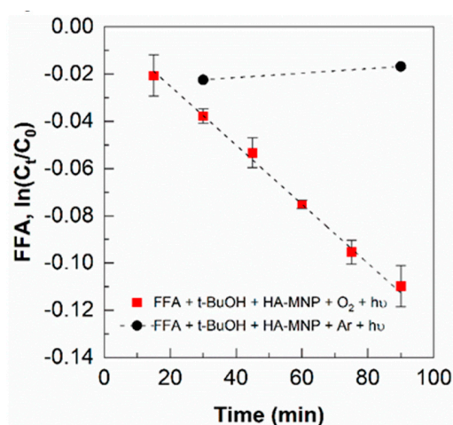
Figure 4. Determination of singlet oxygen generation based on the degradation of FFA, under 350 nm irradiation in the presence of [\text{HA-MNP}] = 1.0 \text{ g L}^{-1} ; [\text{FFA}]_0 = 100 \text{ }\mu\text{M} ; [\text{t-BuOH}] = 10 \text{ mM} , under oxygen-saturated (■) and argon-saturated control experiments (●); error bars represent the standard deviation of triplicate measurements.
