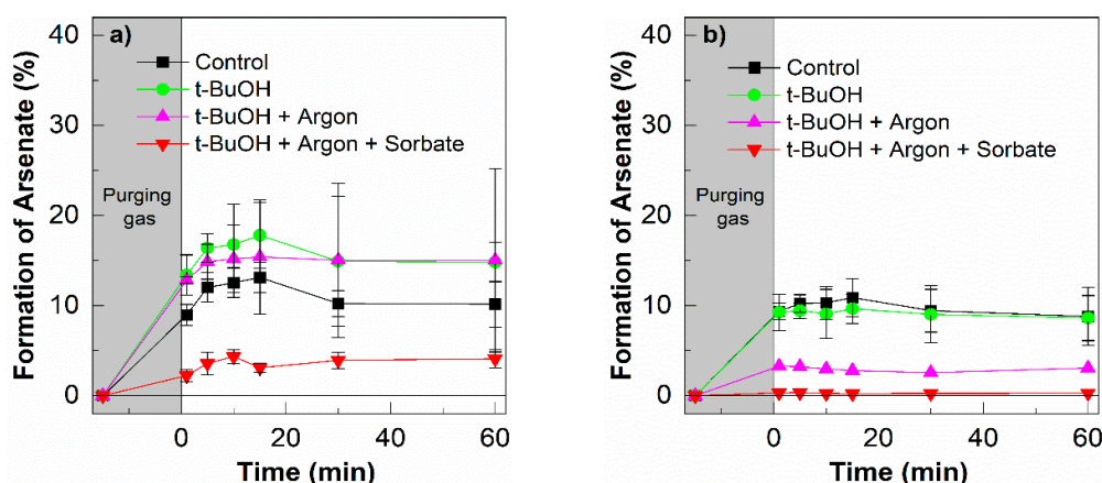
Figure 10. (a) Formation of As(V) in the presence and absence of oxygen, or triplet state quencher sorbate during the photo-irradiation with UVA for 60 min. (b) without UVA. [\text{As(III)}]_0 = 200 \mu\text{g L}^{-1} , [\text{HA} - \text{MNP}] = 0.2 \text{ g L}^{-1} , [t\text{-BuOH}] = 10 \text{ mM} , and [\text{Sorbate}] = 10 \text{ mM} ; error bars represent the standard deviation of triplicate measurements.
