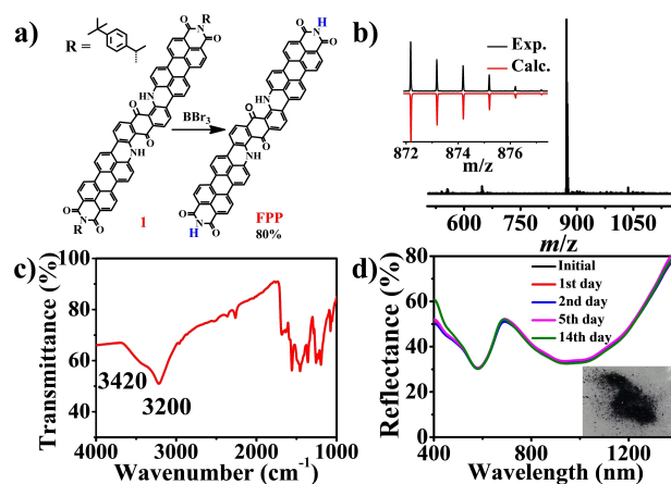
Figure 3. a) De-alkylation reaction from latent pigment 1 to FPP . Reagents and condition: \text{BBr}_3 , dichloromethane, 0^\circ\text{C} , 12 h. b) MALDI-TOF MS of FPP . Inset: experimental and theoretical isotopic distribution patterns. c) FTIR spectrum of FPP . d) Diffuse reflectance spectrum of FPP upon irradiation with sunlight for 14 days under ambient atmosphere. Inset: the photograph of solid powder.
