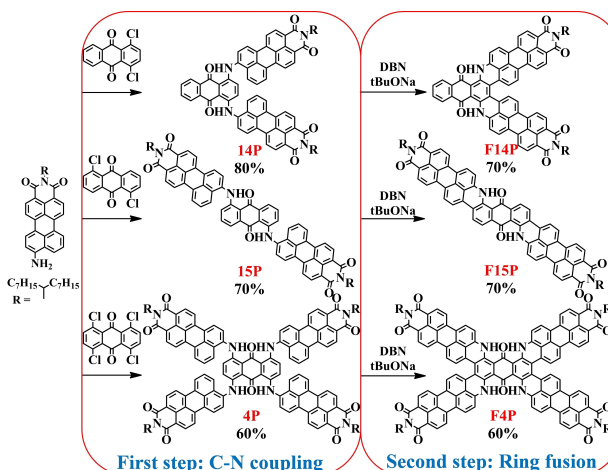
Scheme 2. Synthetic route for FPs. Reagents and conditions of C–N coupling: Brettphos, Brettphos Pd G1, Cs 2 CO 3 , toluene, 110 °C, 12 h, 80% for compound 14P , 70% for 15P , 60% for 4P . Reagents and conditions of dehydrogenative cyclization reaction: DBN, t BuONa, Diglyme, 130 °C, 24 h, 70% for F14P and F15P , 60% for F4P .
