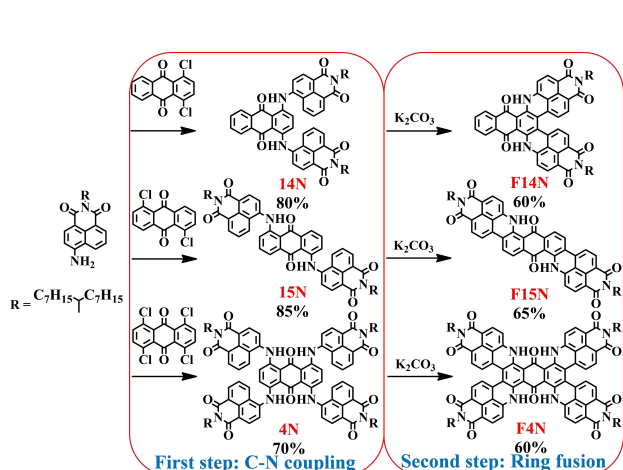
Scheme 1. Synthetic route for FNs. Reagents and conditions of C–N coupling: Brettphos, Brettphos Pd G1, Cs 2 CO 3 , toluene, 110 °C, 12 h, 80% for 14N , 85% for 15N , 70% for 4N . Reagents and conditions of dehydrogenative cyclization reaction: K 2 CO 3 , ethanolamine, 130 °C, 24 h, 60% for F14N , 65% for F15N , 60% for F4N .
