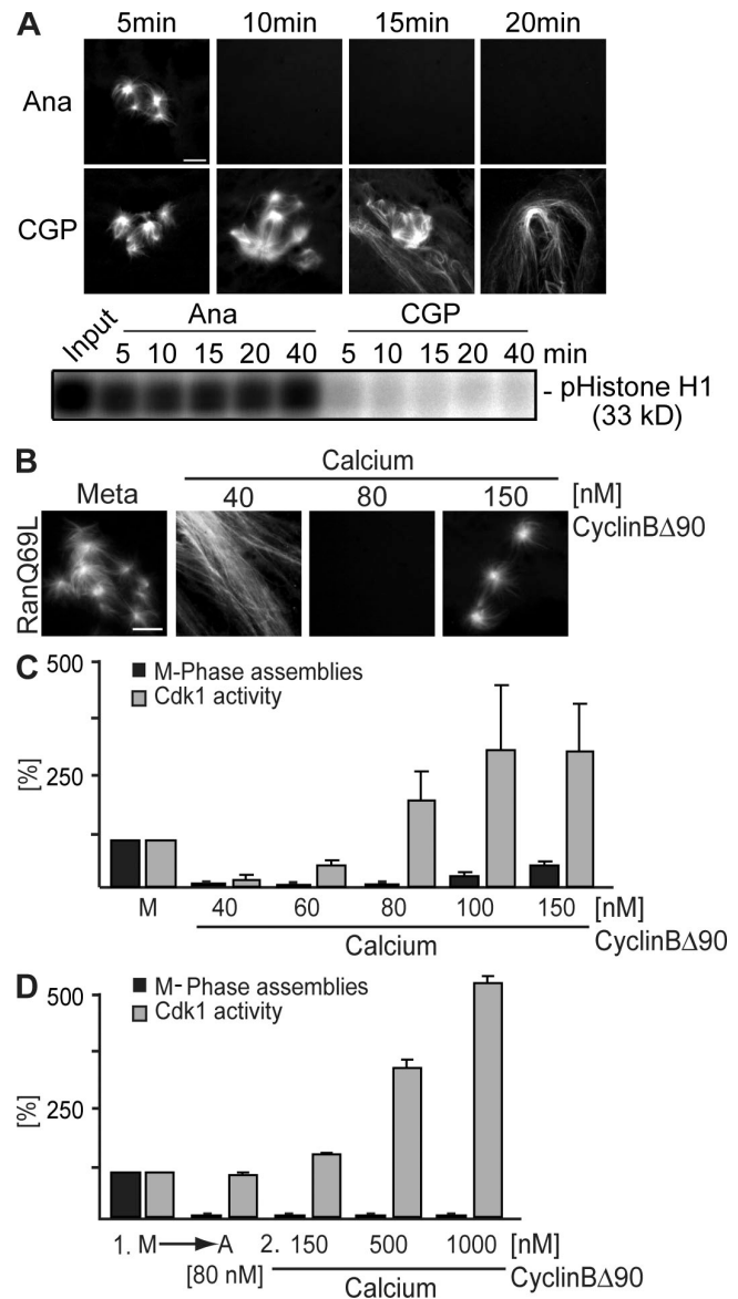
Figure 2. Correlation of Cdk1 activity and changes in microtubule stability at metaphase to anaphase transition. (A) CSF-arrested egg extracts were incubated with calcium and cyclinB \Delta 90 (Ana) or CGP74514A (CGP). Ran-GTP-mediated microtubule assemblies were visualized with calcium fluorescence after the addition of Cy3-labeled tubulin (top), and Cdk1 activities were determined by a histone H1 kinase activity assay (bottom). (B–D) CSF-arrested egg extracts (Meta or M) were triggered to go into anaphase by calcium addition in the presence of increasing cyclinB \Delta 90 concentrations. Ran-GTP-induced metaphase microtubule assemblies were visualized (B) and quantified relative to metaphase as indicated (C, black bars). In parallel, the Cdk1 kinase activity was measured using histone H1 phosphorylation (C, gray bars). (D) Anaphase was first induced with calcium in the presence of 80 nM cyclinB \Delta 90, increasing amounts of cyclinB \Delta 90 were added, and the capacity of Ran-GTP to still induce microtubule assembly was tested. These assemblies were quantified relative to metaphase (black bars), and the Cdk1 kinase activity was measured using histone H1 phosphorylation (gray bars). Error bars represent SD from three independent experiments. Ana, anaphase; Meta, metaphase. Bars, 5 \mu m.
