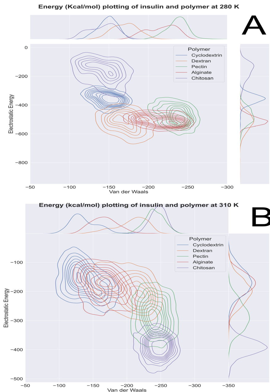
Fig. 8 Molecular dynamics 100 ns insulin-polymer formulation energetics profile at (A) 280 K and (B) 310 K.
