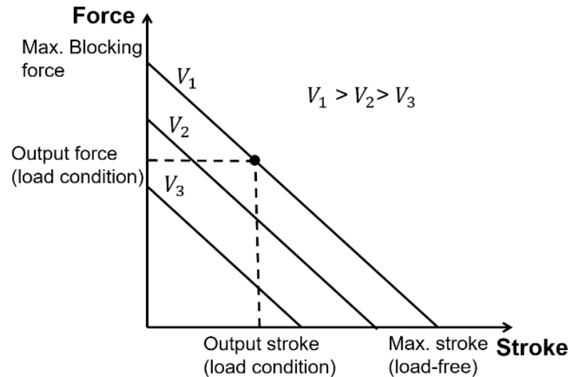
Figure 4. Force–stroke characteristic of the piezoelectric stack.
