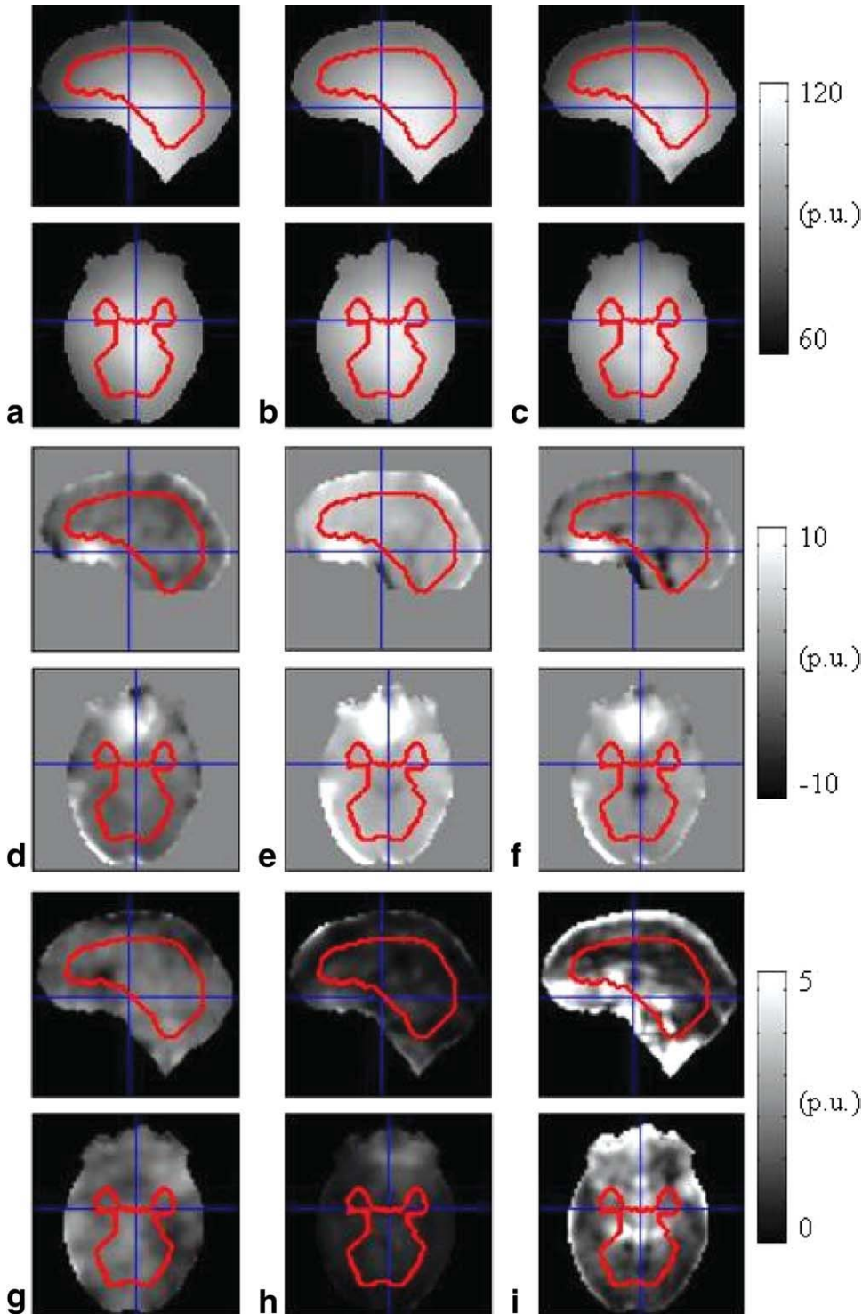
FIG. 3. Sagittal and axial views for a single subject for the 3D AFI ( a,d,g ), 3D EPI ( b,e,h ), and 2D STEAM ( c,f,i ) B_1^+ mapping methods. a-c : B_1^+ maps obtained using each of the methods; ( d-f ) difference images with the reference DAM method; ( g-i ) standard deviation maps taken over four successive repetitions of each method. The red outlines illustrate the ROI used in our study; 164 \times 254 mm ( 600 \times 600 DPI).
