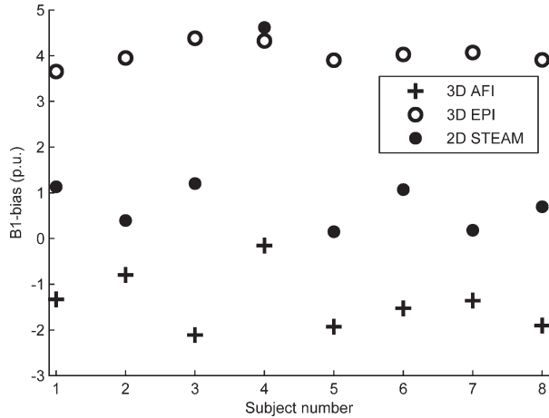
FIG. 4. Bias/accuracy. Flip angle differences between each of the methods under study and the reference DAM technique averaged over the ROI ( B_1 -bias); 103 \times 71 mm ( 600 \times 600 DPI).
