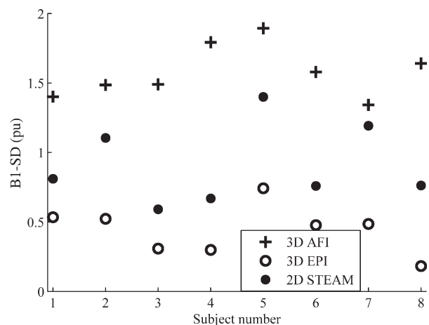
FIG. 5. Reproducibility/precision. Standard deviation of four successive repetitions of each B_1^+ mapping method averaged over the ROI ( B_1 -SD); 103 \times 72 mm ( 600 \times 600 DPI).
