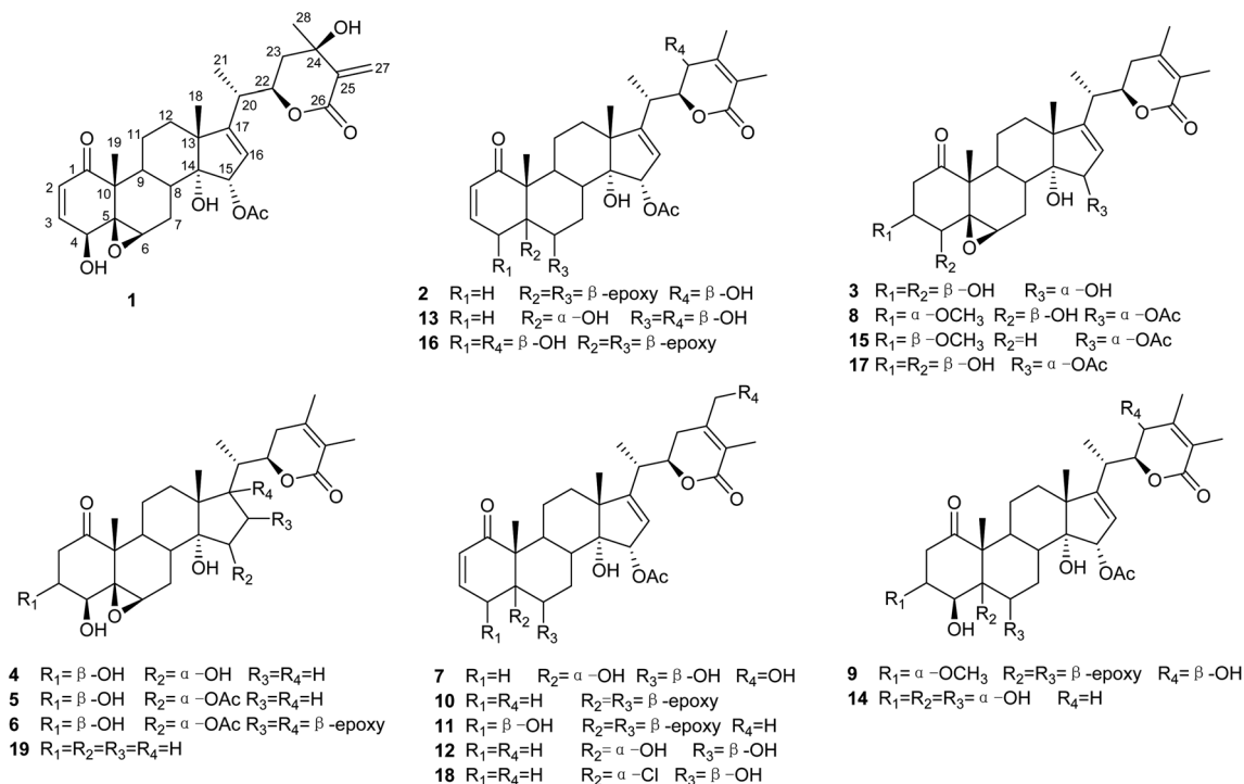
Fig. 1 Structures of compounds 1–19 from Physalis minima .
