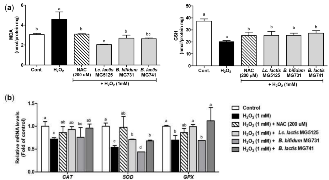
Figure 3. Antioxidant effect of the CFS of probiotics against oxidative stress induced by H 2 O 2 in hepatocytes. (a) MDA and GSH levels in H 2 O 2 -exposed hepatocytes pretreated with the CFS of probiotics. (b) mRNA levels of antioxidant enzymes (CAT, SOD, and GPx) in H 2 O 2 -exposed hepatocytes pretreated with the CFS of probiotics. The cells were pretreated with the CFS of probiotics for 24 h and then exposed to H 2 O 2 (1 mM) for 24 h. Each mRNA level was normalized to the GAPDH . The data represent the mean \pm SEM ( n = 3 ). Different letters among columns indicate significance at p < 0.05 , as determined by Duncan's test. Cont., control; NAC, N -acetylcysteine.
