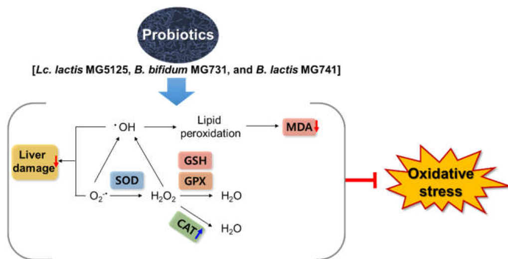
Figure 5. Probiotics exert a hepatoprotective effect by preventing oxidative stress in HepG2 cells and t -BHP-induced mice.
