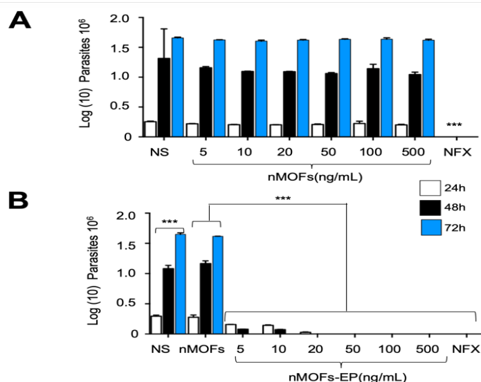
Fig. 3: Effect of MOFs-EP on the growth of tripomastigote forms of T. cruzi . Tripomastigotes were cultured with different concentrations of MOFs-EP for 24–72h, at the end of which the viability of the parasites on the incubations was determined. Values shown are the means \pm SD of triplicate cultures. The data are representative of the results of three independent experiments (*, **, p < 0.001 significantly different from the (control) group untreated (NS), treated with MOFs and NFX at 24 and 48h respectively)
