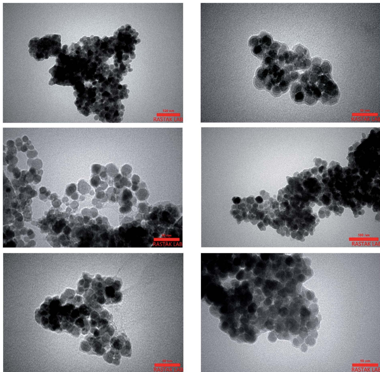
Fig. 4 TEM images of the magnetic \text{Fe}_3\text{O}_4@SiO_2\text{-APTS-EDTA-asparagine} nanomaterial (1).
