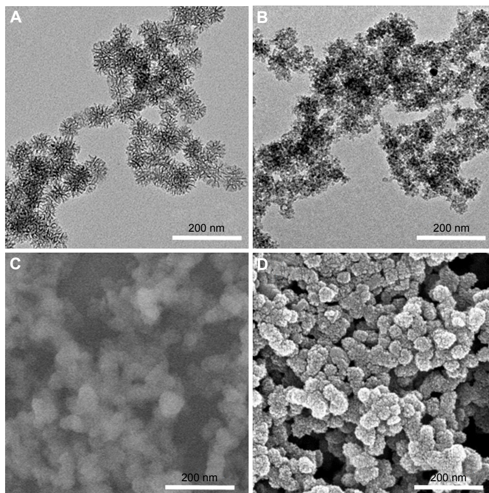
Figure S1 TEM images of (A) MSNs and (B) Ag-MSNs. SEM images of (C) MSNs and (D) Ag-MSNs.
