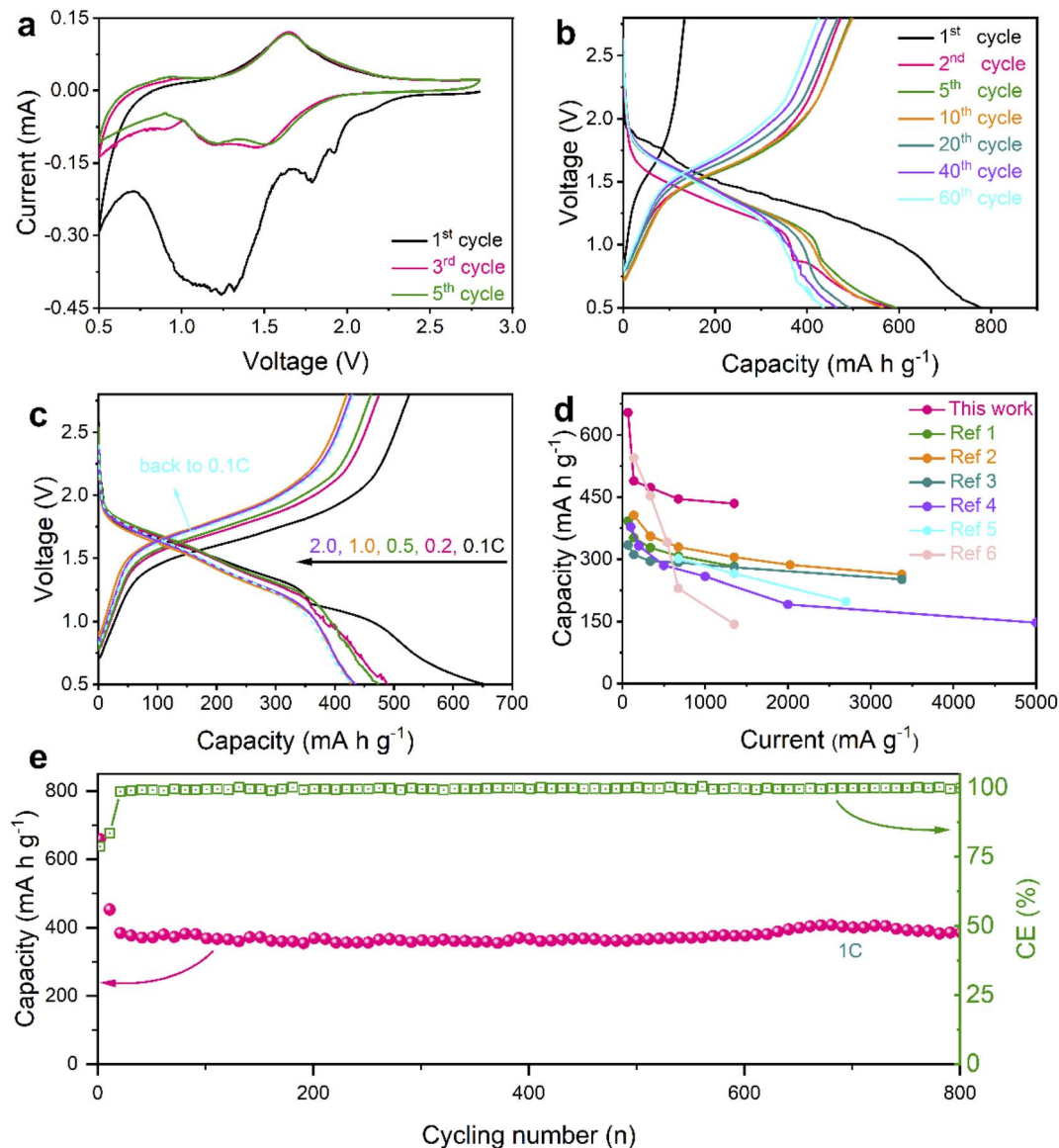
Fig. 4 Electrochemical performance of the Se@THPC composite. (a) CV curves at a scan rate of 0.1 \text{ mV s}^{-1} ; (b) discharge-charge profiles at 0.1C; (c) discharge-charge profiles at various rates; (d) a comparison of rate capabilities between this work and other studies (ref. 1–6 are provided in the ESI†); (e) prolonged cycling stability at 1C.
