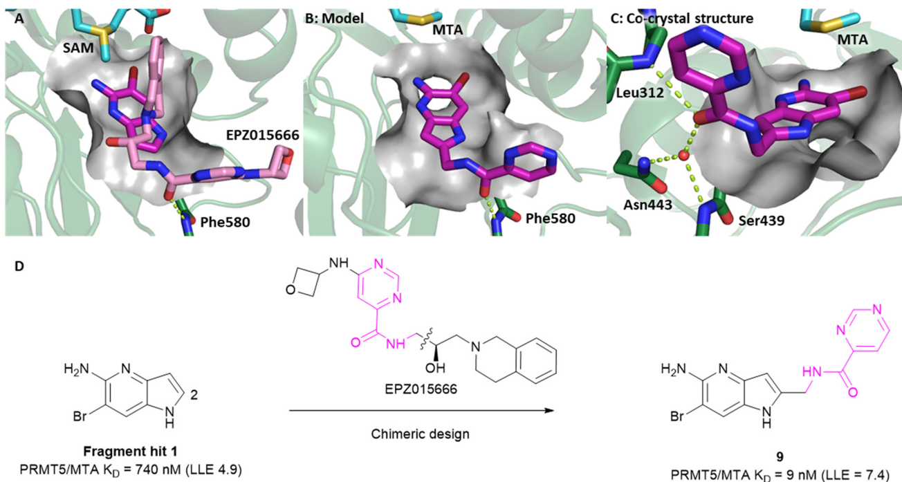
Fig. 8 A) Overlay of fragment hit 1 (magenta) onto the EPZ015666 (pink) PRMT5/SAM X-ray co-crystal structure (PDB: 4X61). B) Model of compound 9 bound in PRMT5/MTA conceived by the overlay of fragment hit 1 and EPZ015666. C) X-ray co-crystal structure of 9 bound to PRMT5/MTA (PDB: 7ZUQ). 9 adopts an alternative conformation to the model forming an H-bond between the amide carbonyl of 9 and Leu312 and water mediated H-bonds to Asn443 and Ser439. D) SBDD enabled optimization of fragment hit 1 to give compound 9.
