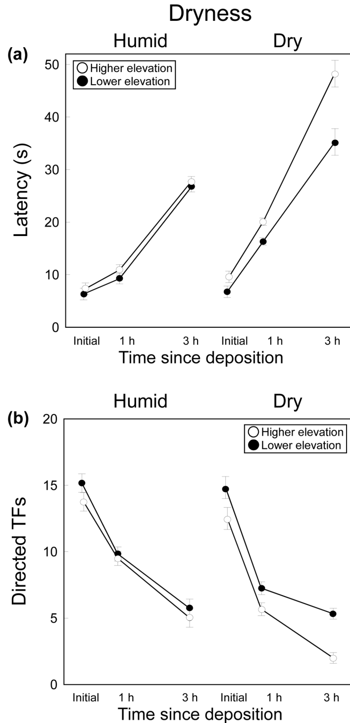
Fig 3. Effects of Dryness on Signal Efficacy. Mean \pm SE (a) latency and (b) number of tongue-flicks (TF) directed to swabs by female P. hispanicus lizards from two populations (lower elevation: black; higher elevation: white) in response to swabs bearing femoral secretions of males immediately after they were secreted ('initial'), 1 h or 3 h since deposition and maintained under two dryness conditions (humid vs. dry).
