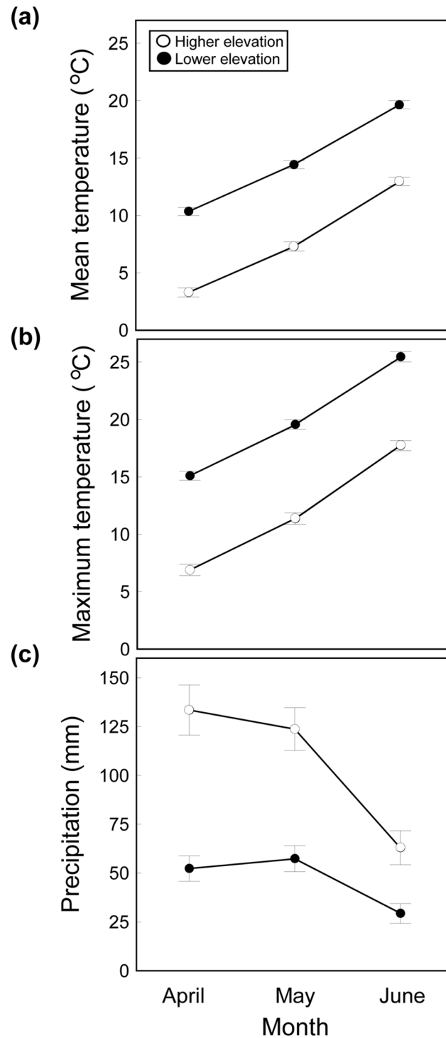
Fig 1. Climatic Conditions at the Lizards' Populations. Variation in (a) daily mean and (b) daily maximum air temperatures, and (c) total monthly precipitation in two populations (lower elevation: black circles; higher elevation: grey circles) of the Guadarrama Mts., Central Spain, in the months of April, May and June, coinciding with the mating season of Podarcis hispanicus lizards. Data show average ( \pm SE) monthly values for a 34 years period (1978–2011).
