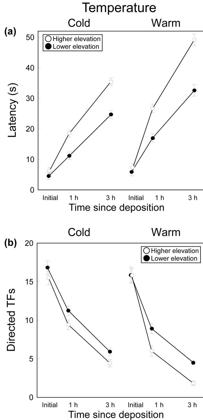
Fig 2. Effects of Temperature on Signal Efficacy. Mean \pm SE (a) latency and (b) number of tongue-flicks (TF) directed to swabs by female P. hispanicus lizards from two populations (lower elevation: black; higher elevation: white) in response to swabs bearing femoral secretions of males immediately after they were secreted ('initial'), 1 h or 3 h since deposition and maintained under two temperature regimes (cold vs. warm).
