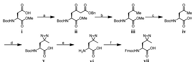
Scheme 1 Synthesis of Fmoc-photo-Leu; conditions: (a) 1,1'-carbonyldiimidazole, isopropyl magnesium chloride, monobenzyl malonate, THF, 85%; (b) Pd/C, MeOH, 83%; (c) LiOH, THF/H 2 O (2 : 1), r.t., 98%; (d) (1) NH 3 , hydroxylamine- O -sulfonic acid; (2) TEA, I 2 , MeOH, 30%; (e) TFA/dichloromethane (1 : 1); (f) Fmoc-OSu, NaHCO 3 , 1,4-dioxane/H 2 O (2 : 1), 97% over two steps.
