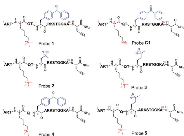
Fig. 1 Chemical structures of photoaffinity probes 1 – 5 and C1 .
