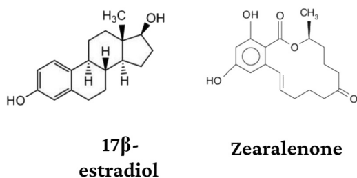
Fig. 1. Chemical structure of Estrogen (17 \beta - estradiol) and Zearalenone.
