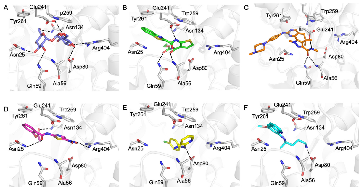
Fig. 5 In silico analysis of Pathogen Box hit compounds with LpqY. A) Trehalose (blue carbon atoms), B) TCA1 (green carbon atoms), C) milcliclib (orange carbon atoms) D) nitazoxanide (magenta carbon atoms), E) MMV676524 (yellow carbon atoms), F) primaquine (cyan carbon atoms). LpqY is shown in cartoon format and residues are shown in grey. Dashed lines represent hydrogen bonds.
