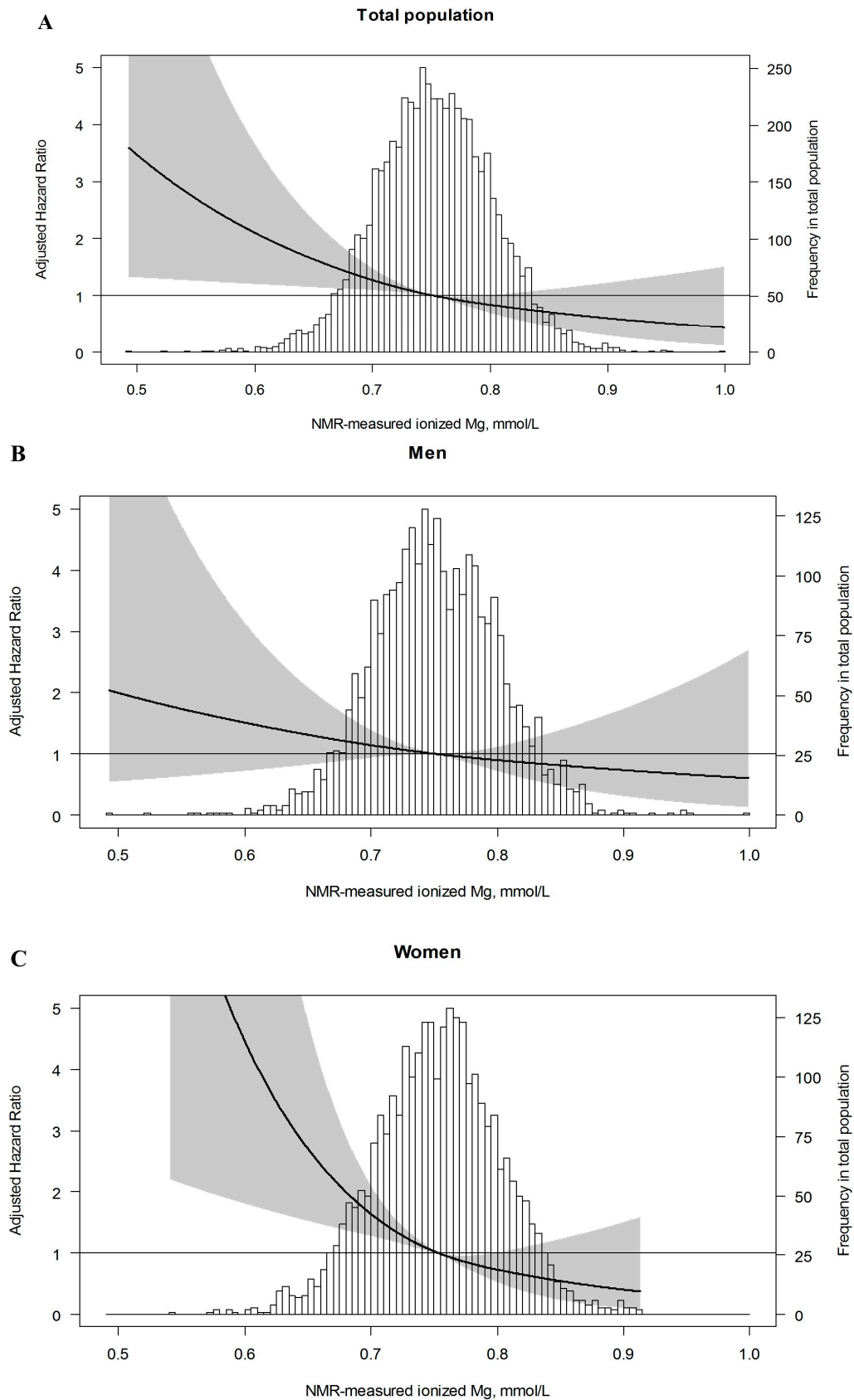
Figure 4. Association between NMR-measured Mg and the risk of developing T2DM. Data were fit by a restricted cubic spline with 3 knots and were adjusted for age (A–C) and sex (A).
