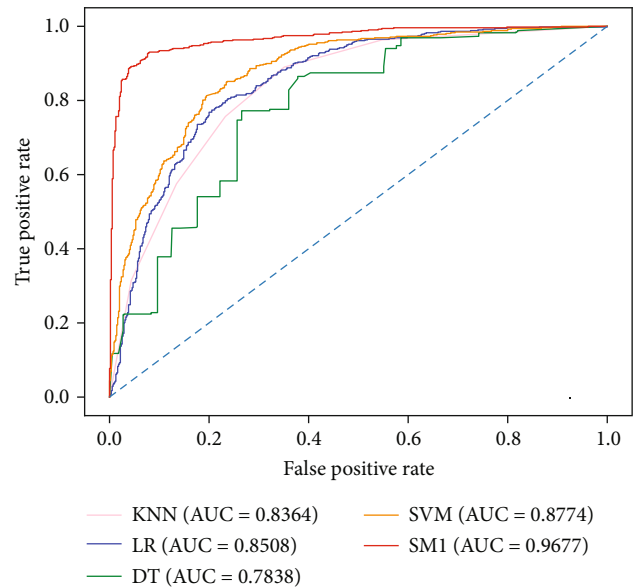
FIGURE 4: ROC curves of SM1 and its base classifiers on the PDB1075 dataset.
