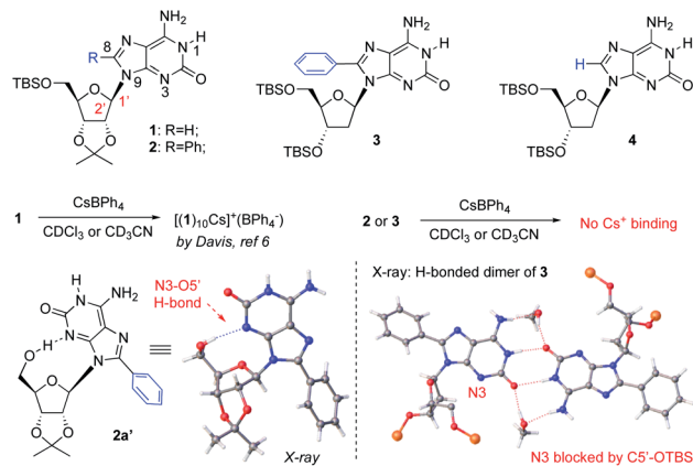
Fig. 1 Challenge of isoG-star formation using isoG derivatives.
