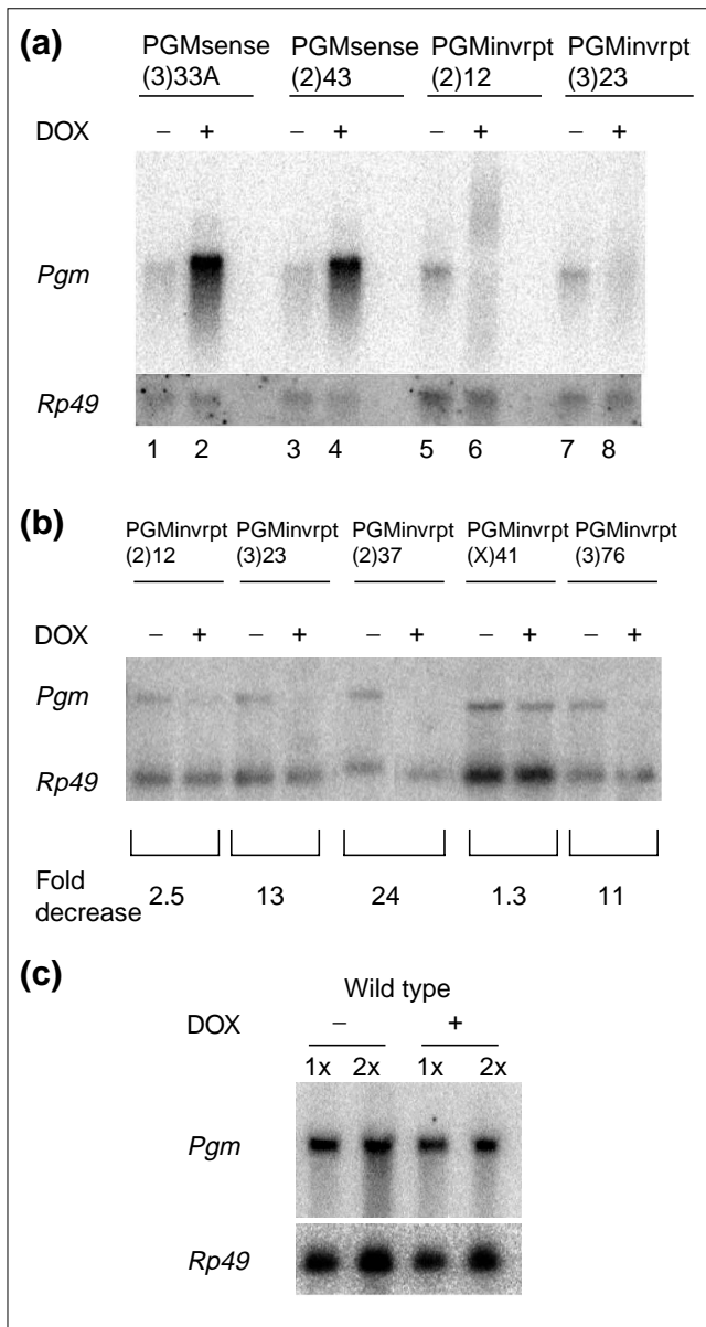
Figure 3 Northern analysis of PGMsense and PGMinvrpt construct lines. Total RNA was isolated from adult males of the indicated PGMsense lines, PGMinvrpt lines, and control line, with or without DOX treatment. (a) Northern blot hybridized with a probe that will recognize both endogenous and transgenic Pgm transcripts and with a probe specific for Rp49 as a loading control. (b) Northern blot hybridized with a probe that will recognize only the endogenous Pgm transcript and with a probe specific for Rp49 as a loading control. The fold decrease in Pgm transcript abundance is indicated below the lanes. (c) Northern blot of control strain hybridized with a probe that will recognize the endogenous Pgm transcript and with a probe specific for Rp49 as a loading control.
