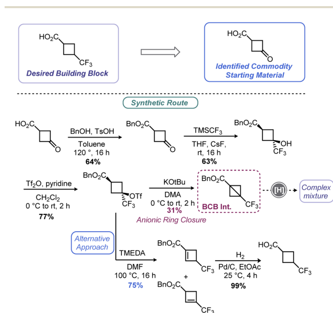
Scheme 14 Merck's approach to a cyclobutyl building block via a BCB intermediate.
